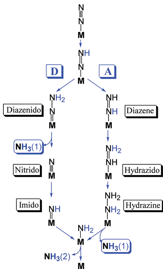
FIGURE 4. “Alternating” (A) and “distal” (D) N_2 reduction pathways. M represents FeMo-co without specifying metal ion(s) involved. Likewise, the representations of binding are meant to emphasize the distinction between pathways and do not imply specific binding modes. Small straight arrows represent addition of H^+/e^- to substrate.
