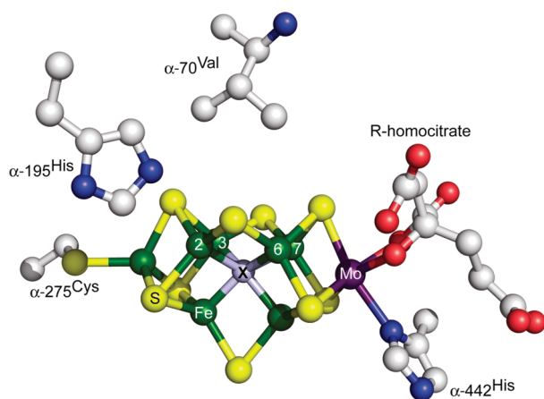
FIGURE 2. Structure of FeMo-co, including the two residues that covalently link it to the apoprotein and the two implicated in function, \alpha -V70 as substrate “gatekeeper” and \alpha -H195 as agent for proton delivery.
