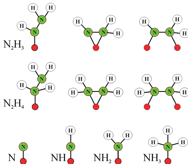
CHART 1. Substrate-Derived Species Bound to FeMo-co That Might Form in Late Stages of \text{N}_2 Reduction
