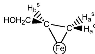
FIGURE 3. Proposed structure for the intermediate trapped during propargyl alcohol reduction, the product alkene bound side-on to a single Fe ion.
